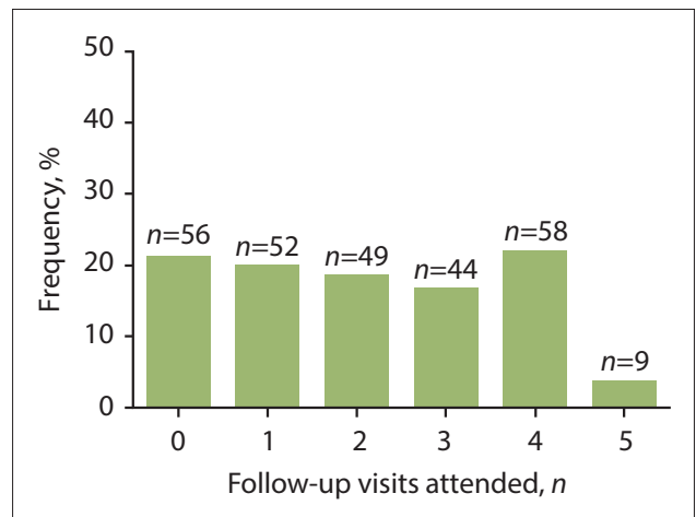
Fig. 4. Frequencies (%) of the number of follow-up visits that participants (N=268) attended. Patients were divided into six groups, based on their follow-up status: those who attended none of the five follow-up visits were grouped into group 0 ( n=56 ), those who attended all follow-up visits were grouped into group 5 ( n=9 ), and those who attended only a subset of scheduled follow-up visits were grouped into groups 1 - 4. The total number of participants in each follow-up group is indicated.
