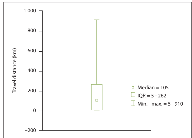
Fig. 3. Box-and-whisker plot indicating the median travel distance (105 km) with IQR (5 - 262 km) and minimum/maximum distances (5 - 910 km) travelled. (IQR = interquartile range; min. = minimum; max. = maximum.)
